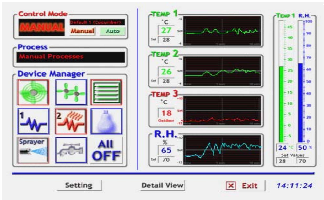
Fig. 4. Main graphical user interface of the Greenhouse Control & Monitoring Software
