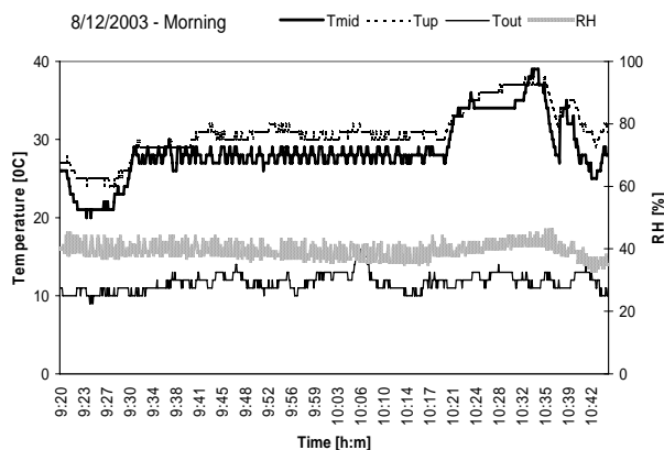
Fig 7. Measured temperatures and relative humidity under the action of controller: (a) Temperature control (left), and (b) Temperature and RH control (right)
