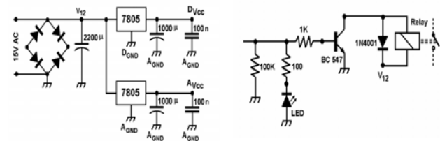
Fig. 3. Electronic circuitry for (a) power supply (left) and (b) relay activation (right)
