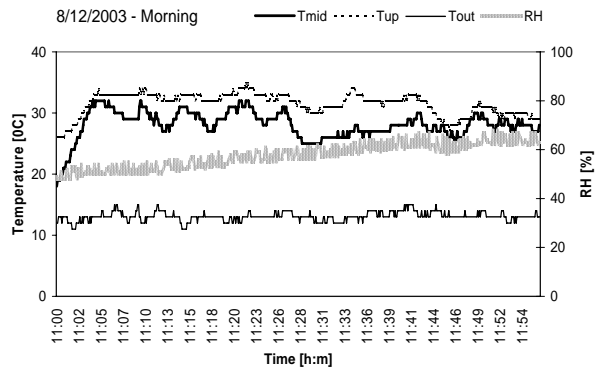
Fig 7. Measured temperatures and relative humidity under the action of controller: (a) Temperature control (left), and (b) Temperature and RH control (right)
