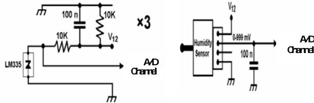
Fig. 2. Conditioning circuits for (a) temperature (left) and (b) humidity measurements (right)
