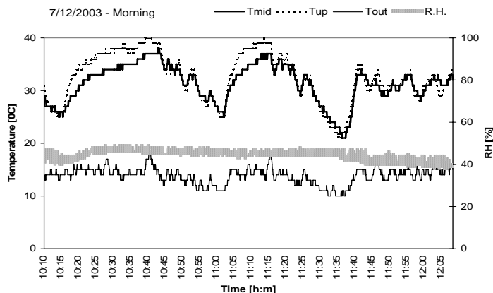
Fig. 6. Measured temperatures and relative humidity in no-control operation
