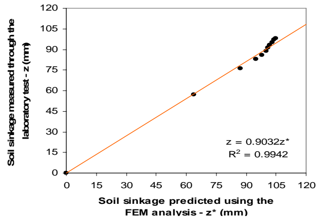
Fig. 8: Soil sinkage values predicted using the FEM analysis and soil sinkage values measured through the laboratory test are plotted against each other and fitted with a linear equation with zero intercept
