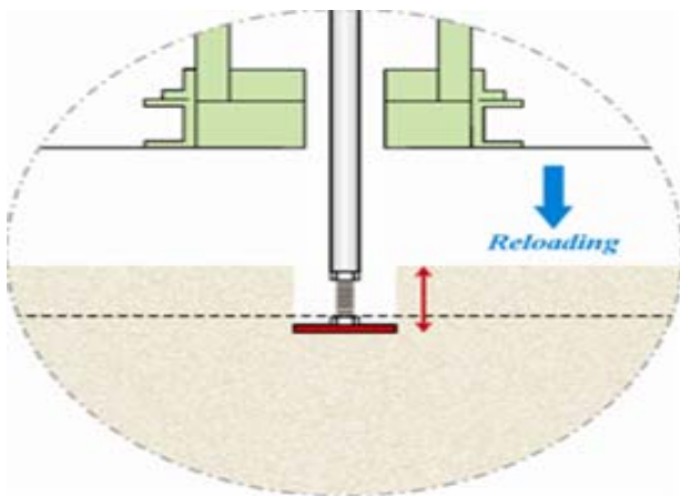
Fig. 5: Reloading process
