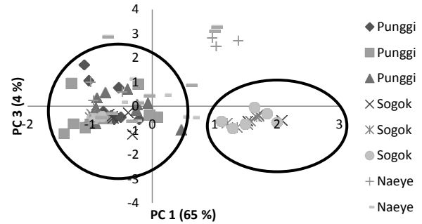
Fig. 5: Biplots of PC 1 and PC 3 extracted from the principal component analysis (PCA) of the carbon utilization profile at 96 h of incubation of Biolog EcoPlate™. Points within a group have comparable microbial structures
