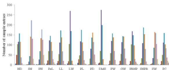
Fig. 3: Distribution diagram of subordinate function value of fifteen phenotypic traits
