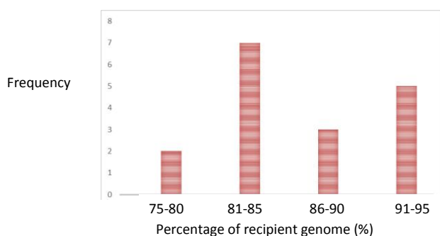
Fig. 2: Frequency distribution of recurrent parent genome recovery (%) in BC 1 F 1 population
