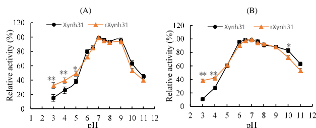
Fig. 5: The effect of pH on the endoxylanase (A) Optimum reaction pH of the endoxylanase. (B) The pH stability of the endoxylanase
