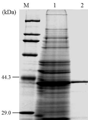
Fig. 1: SDS-PAGE of purified Xynh31 M: Premixed Protein Marker; 1: Crude enzyme; 2: SP-Sepharose Fast Flow Enzyme activity fraction
