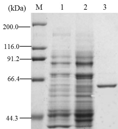
Fig. 3: SDS-PAGE of the expression and purified endoxylanase M: Premixed Protein Marker (High); 1: Without IPTG; 2: Induction with 0.2 mM IPTG; 3: Purified protein
