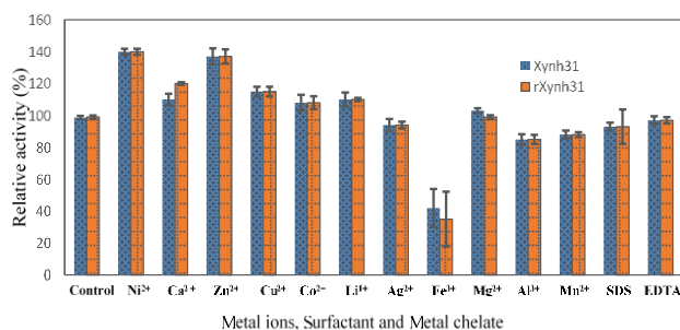
Fig. 6: Effect of metal ions, surfactant and metal chelate on endoxylanase activity
