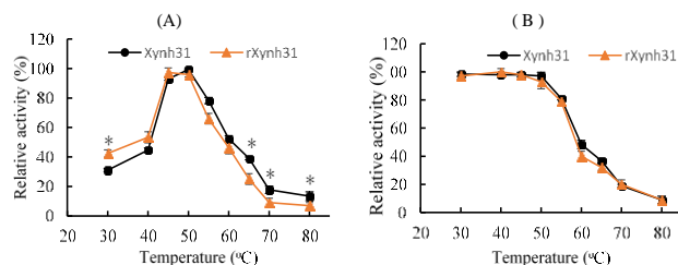
Fig. 4: The effect of temperature on the endoxylanase (A) Optimum reaction temperature of the endoxylanase. (B) Thermostability of the endoxylanase
