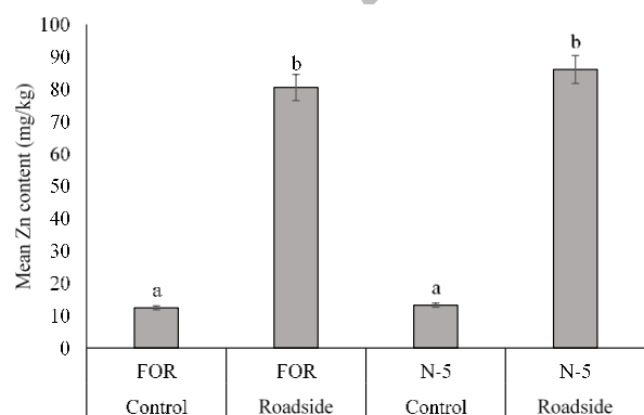
Fig. 9: Comparison among roads for mean Zn contents (mg kg -1 dry wt.) in plant leaves
