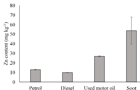
Fig. 10: Zinc content in fuel and soot (mg kg -1 )
