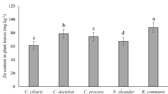
Fig. 3: Mean of Zn content (mg kg -1 dry wt.) in plant leaves along "N-5"
