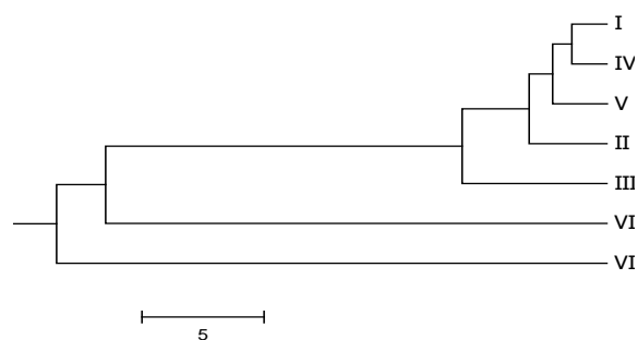
Fig. 3: UPGMA cluster graph of 7 groups
