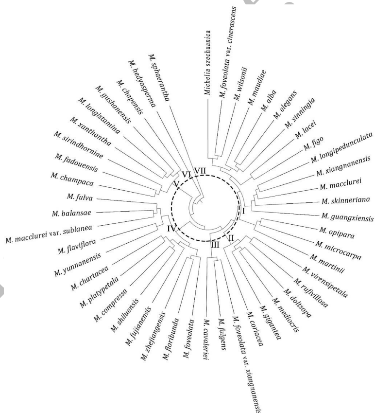
Fig. 2: UPGMA cluster map of 48 species of Michelia
