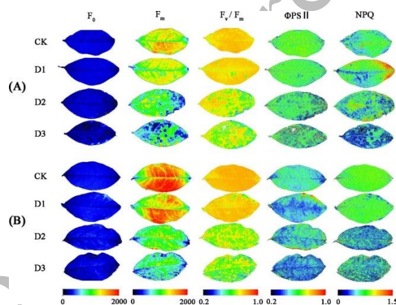
Fig. 4: Changes in chlorophyll fluorescence parameters F_0 , F_m , F_v/F_m , \Phi_{PSII} and NPQ images of CK, D1, D2 and D3 treatments in Longjing43 (A) and Yingshuang (B) tea plants. F_0 , F_m , F_v/F_m , \Phi_{PSII} and NPQ indicate the minimum fluorescence, maximal fluorescence, maximum quantum efficiency of PSII, effective photochemical quantum yield of PSII, and non-photochemical quenching
