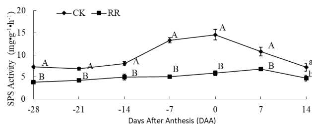
Fig. 9: Effects of root restriction on the SPS activity of tree peony leaves
