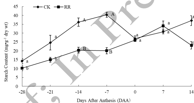
Fig. 6: Effects of root restriction on the starch content of tree peony leaves
