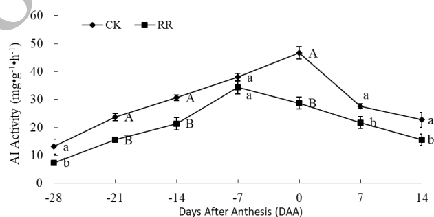
Fig. 7: Effects of root restriction on the AI activity of tree peony leaves
