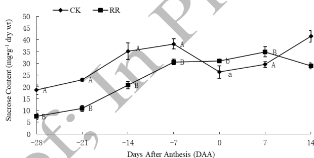
Fig. 2: Effects of root restriction on the sucrose content of tree peony leaves
