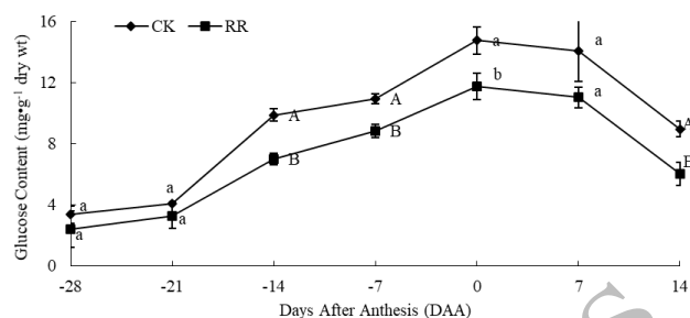
Fig. 5: Effects of root restriction on the glucose content of tree peony leaves
