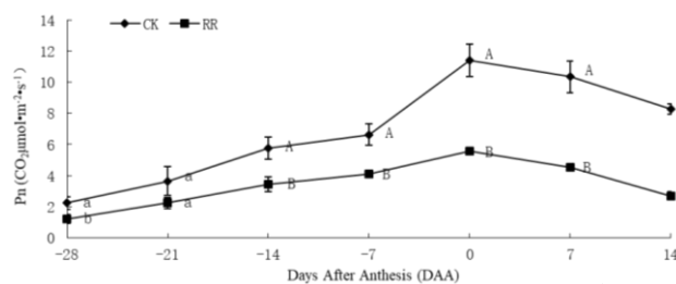
Fig. 1: Effects of root restriction on the Pn of tree peony leaves (aa, ab and AB above the standard error bars indicate that there is no significant difference, the difference is significant at P < 0.05 level, and the difference is significant at P < 0.01 level. The same as below)
