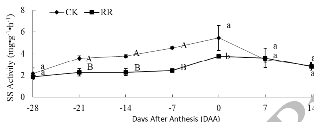
Fig. 10: Effects of root restriction on the SS activity of tree peony leaves
