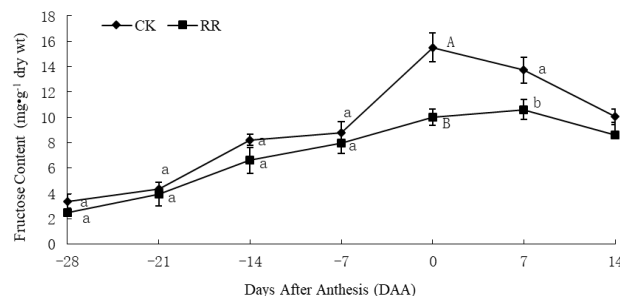
Fig. 4: Effects of root restriction on the fructose content of tree peony leaves
