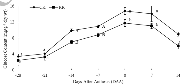
Fig. 3: Effects of root restriction on the glucose content of tree peony leaves
