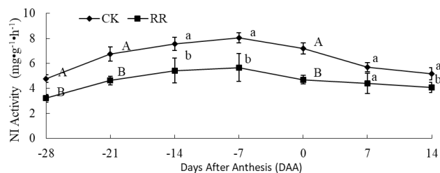
Fig. 8: Effects of root restriction on the NI activity of tree peony leaves
