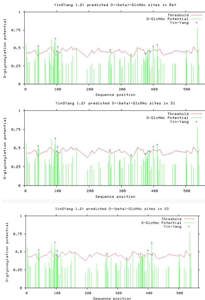
Fig. 3: Graphical representation of Prediction of Potential Glycosylation and YinOYang sites in N. crassa (A), SFS strains (B) and NFS strains (C) of S. fimicola at 0.5 thresholds
