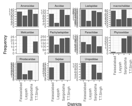
Fig. 3: Community Structure of Mesostigmata during different months
