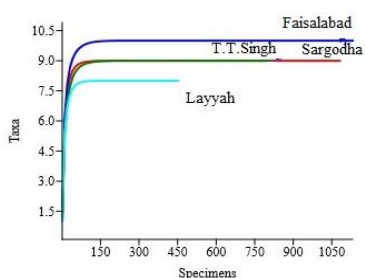
Fig. 1: Rarefaction curve for cumulative data of citrus orchards of Punjab
