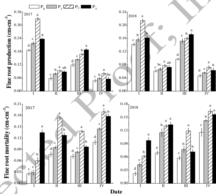
Fig. 5: Fine root production and mortality of alfalfa in different treatments ( \text{cm}\cdot\text{cm}^{-3} )
