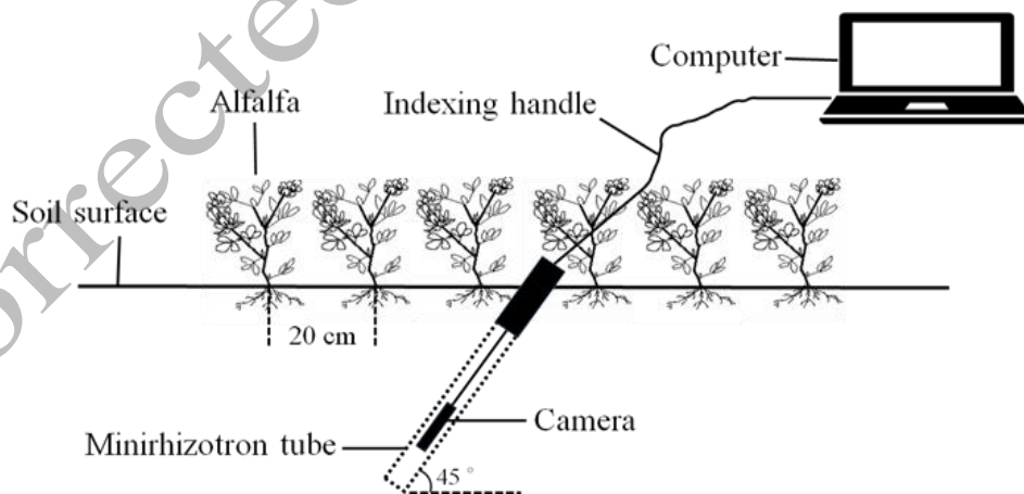
Fig. 2: Minirhizotrons installation
