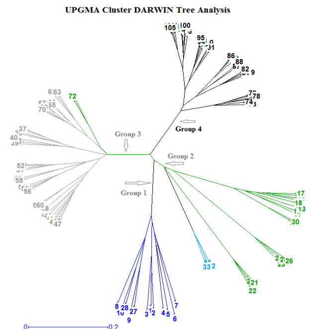
Fig. 3: UPGMA DARWIN tree displaying the distribution of the 105 bread wheat genotypes in four groups, and presenting the genetic similarities and dissimilarities within and between the groups
