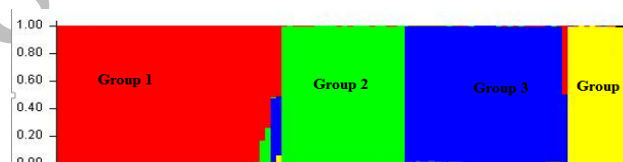
Fig. 4: Population structure of 105 bread wheat genotypes based on Bayesian method analyzed with 302 polymorphic SSRs detecting 4 groups. The dissimilar colors in this figure demonstrating the different group
