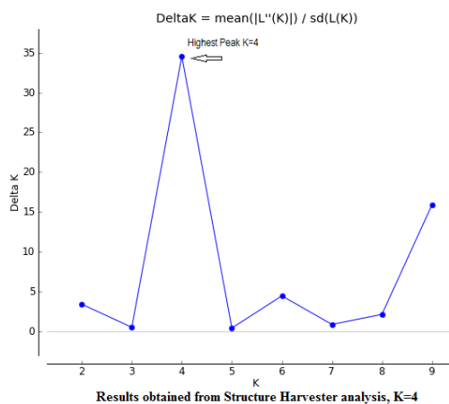
Fig. 2: This result achieved of 105 bread wheat genotypes using 302 polymorphic SSR markers from Structure Harvester analysis. It's based on the second order derivation on the variance of the maximum likelihood estimation of your model given a specific K. Delta K shows only the uppermost clustering level and number of subpopulations in main population
