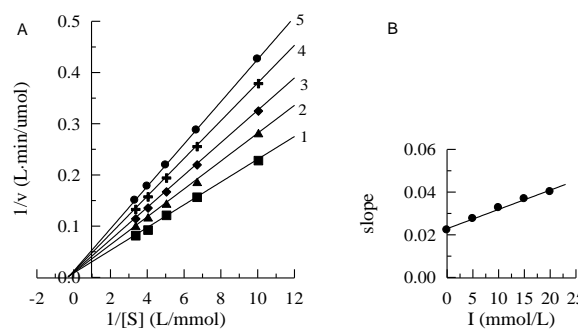
Fig. 3: Lineweaver-Burk Plots for the NAGase inhibition by acetamide (A) Plots 1–5 correspond to results using acetamide concentrations of 0, 5, 10, 15, and 20 mmol/L, respectively
