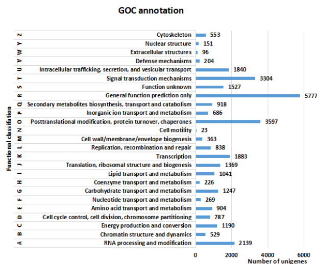
Fig. 3: KOG functional classification of Vaccinium uliginosum Unigenes
