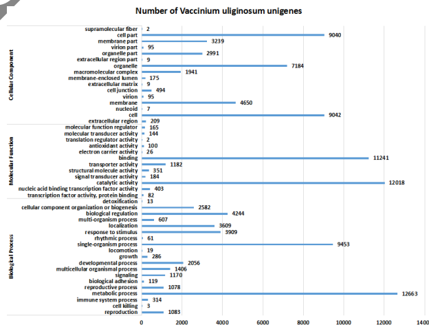
Fig. 2: GO functional classification of Vaccinium uliginosum Unigenes
