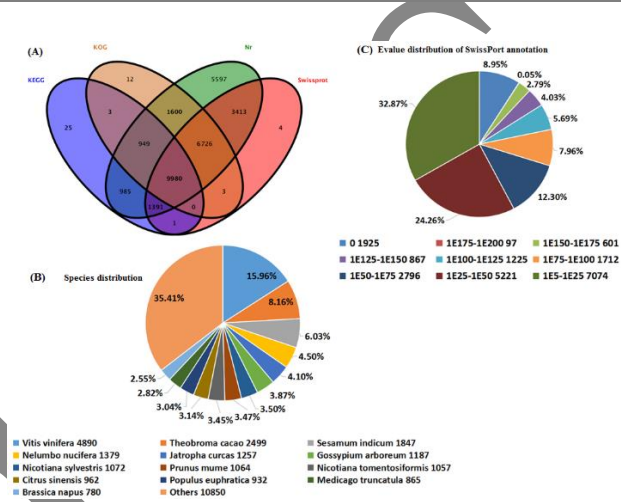
Fig. 1 (A): Venn diagram of BLAST hits for unigenes against KOG, Nr, Swiss-Port and KEGG database (E-value≤1.0e-05). Numbers in the circles indicate the number of unigenes annotated by single or multiple databases, (B) Species distribution of the top BLAST hits for the assembled unigenes (E-value of 1.0e-05). (C) E-value distribution of BLAST hits Swiss-Port dataset for each unique sequence (E-value ≤1.0e-05)
