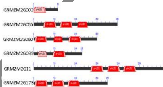
Fig. 1: Systematic evolution of the LSD genes in maize and Arabidopsis
