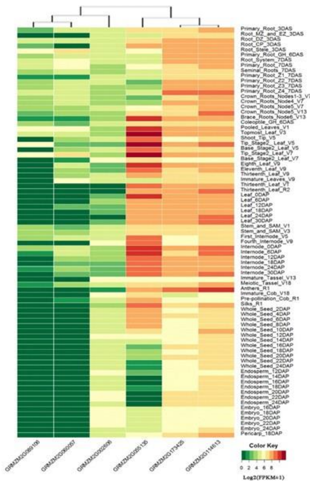
Fig. 4: Expression pattern of LSD in maize
