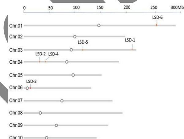
Fig. 3: Location of LSD genes on chromosomes of maize
