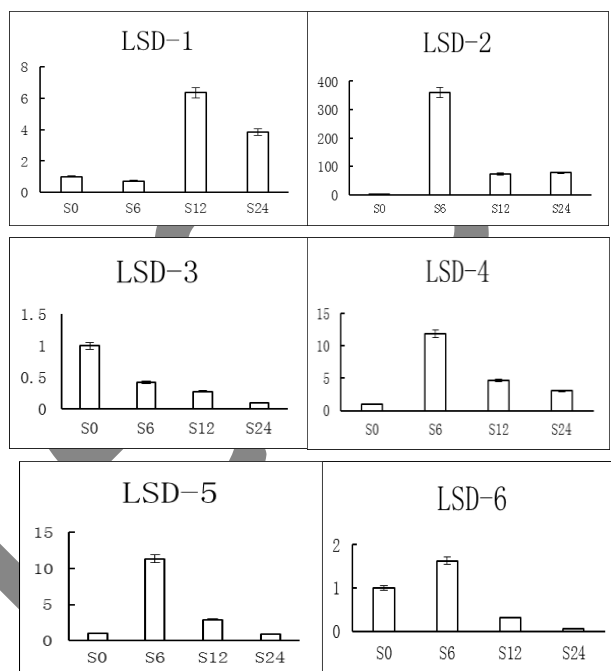
Fig. 5: Expression level of LSD after Fusarium graminearum infecting
