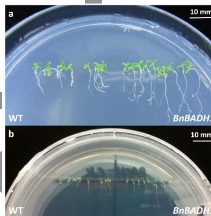
Fig. 5: Enhanced tolerance to drought or salt stress
