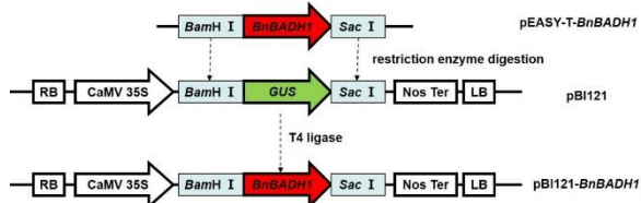
Fig. 1: Strategy for construction of overexpressing vector of pBI121- BnBADHI
