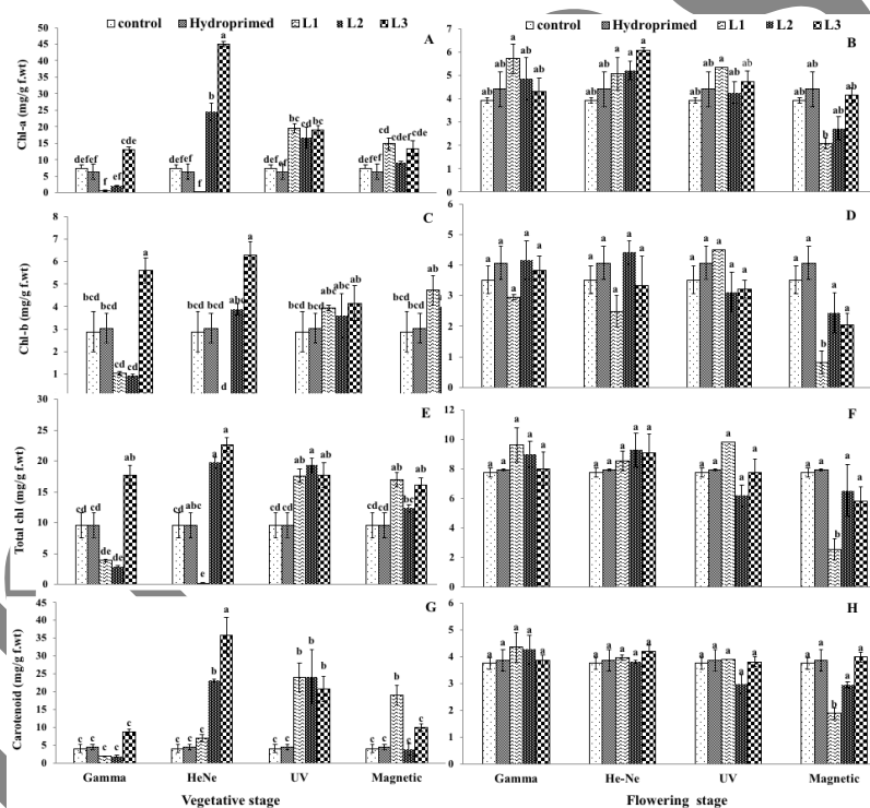
Fig. 1: Effect of pre sowing seed treatment with selected physical agents on pigmentation in sunflower. Means with same letters, for each trait, do not differ significantly from each other at p \leq 0.05 . For magnetic field L1= 0.1 Tesla, L2= 0.2 Tesla, L3=0.3 Tesla, for ultraviolet (L1= 20 min, L2=40 min, L3= 60 min.), for He-Ne laser treatment (L1= 1 min, L2= 2 min, L3= 3 min), for gamma ( \gamma ) irradiation (L1= 10 kGy, L2=20 kGy, L3= 30 kGy). A, C, E, G corresponds to Chlorophyll a, b, total chlorophyll and carotenoid contents at vegetative stage while B, D, F, H corresponds to Chlorophyll a, b, total chlorophyll and carotenoid contents at flowering stage
