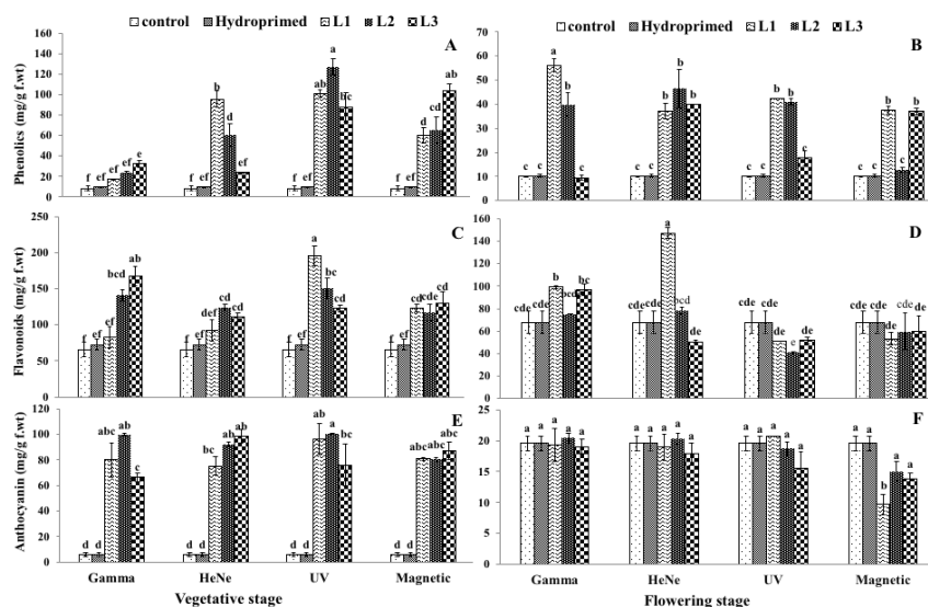
Fig. 3: Effect of pre sowing seed treatment with selected physical agents on secondary metabolites in sunflower. Means with same letters, for each trait, do not differ significantly from each other at p \leq 0.05 . For magnetic field L1= 0.1 Tesla, L2= 0.2 Tesla, L3=0.3 Tesla, for ultraviolet (L1= 20 min, L2=40 min, L3= 60 min), for He-Ne laser treatment (L1= 1 min, L2= 2 min, L3= 3 min), for gamma ( \gamma ) irradiation (L1= 10 kGy, L2=20 kGy, L3= 30 kGy). A, C, E corresponds to Phenolics, Flavonoids and Anthocyanin at vegetative stage while B, D, F corresponds to Phenolics, Flavonoids and Anthocyanin at flowering stage
