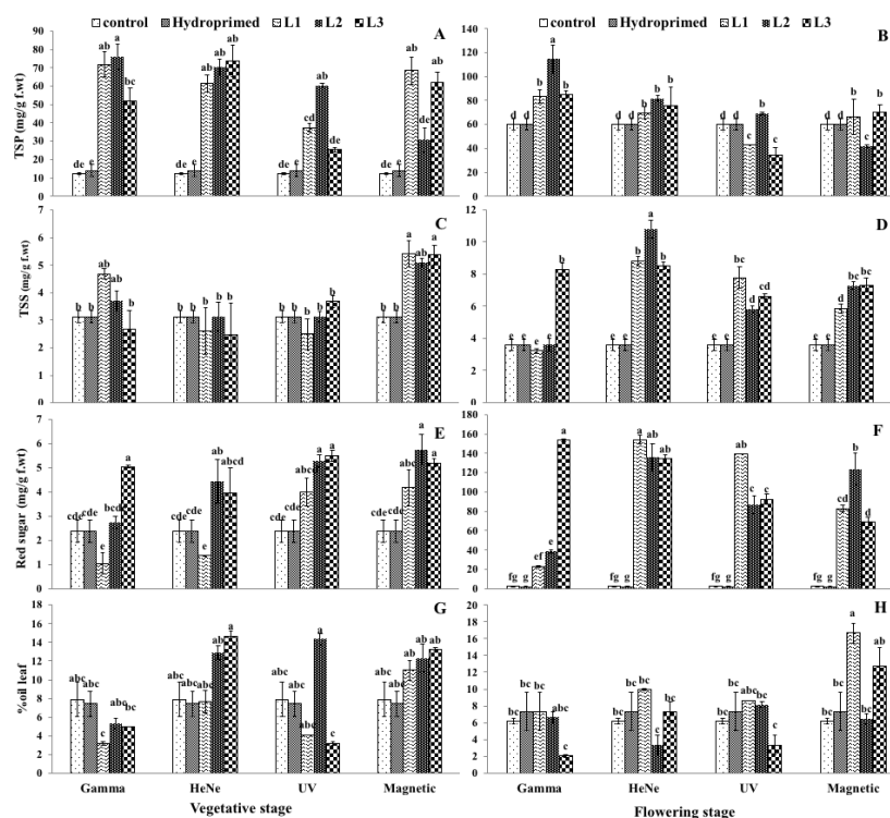
Fig. 2: Effect of pre sowing seed treatment with selected physical agents on primary metabolites in sunflower. Means with same letters, for each trait, do not differ significantly from each other at p \leq 0.05 . For magnetic field L1= 0.1 Tesla, L2= 0.2 Tesla, L3 = 0.3 Tesla, for ultraviolet (L1= 20 min, L2=40 min, L3= 60 min), for He-Ne laser treatment (L1= 1 min, L2= 2 min, L3= 3 min), for gamma ( \gamma ) irradiation (L1= 10 kGy, L2=20 kGy, L3= 30 kGy). A, C, E, G corresponds to Total soluble proteins (TSP), Total soluble sugars (TSS), Reducing sugars and Leaf percentage oil contents at vegetative stage while B, D, F, H corresponds to Total soluble proteins (TSP), Total soluble sugars (TSS), Reducing sugars and Leaf percentage oil at flowering stage
