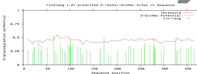
Fig. 1: Graphical representation of glycosylation potential of CyC1 protein in N. crassa and S. fomicola (S 1 , S 2 , S 3 , N 5 , N 6 , N 7 ). Red zigzag line shows the threshold (0.5), green lines shows the O-glycosylation potential. Green lines exceeding threshold shows the positions of glycosylation
