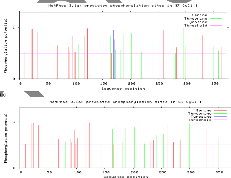
Fig. 2: Graphical representation of phosphorylation potential of CyC1 protein (a) In N. crassa , N 5 , N 6 and N 7 (b) In S 1 , S 2 and S 3 . Red Lines= Serine, Green Lines= Threonine, Blue Lines= Tyrosine and Pink Line= Threshold. Lines exceeding pink line (threshold= 0.5) shows the positions of phosphorylation in CyC1 and red, green, blue color of lines shows the residue present at that position
