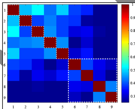
Fig. 3: Klee diagram for the COI gene. Color gradation in red indicates strong correlation (high correlation value). Red blocks in white dashed box indicate sequences of E. fabae , E. luda , E. coccinea , E. decipiens , E. onukii and outgroups 1. E. fabae ; 2. E. luda ; 3. E. coccinea ; 4. E. decipiens ; 5. E. onukii ; 6. Amrasca biguttula ; 7. Anaka burmensis ; 8. Thampos dansaiensis ; 9. Typhlocyba rosae
