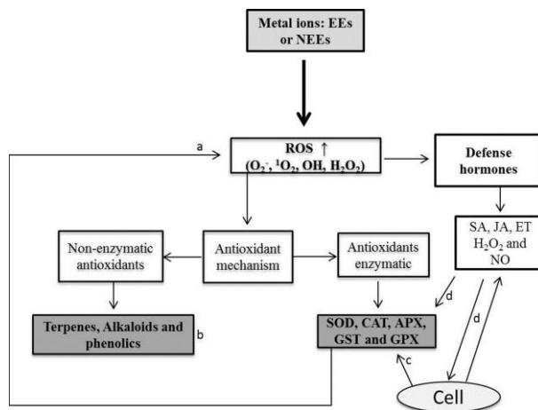
Fig. 1: Metal ion signaling pathway and specific response mechanism: a) degradation/accumulation; b) activation/deactivation of compounds; c) activity increase or decrease; d) regulation of antioxidant enzymes. EEs: essential elements; NEEs: non-essential elements; ROS: reactive oxygen species; SOD: superoxide dismutase; CAT: catalase; APX: ascorbate peroxidase; GST: glutathione S-transferase; GPX: glutathione peroxidase; SA: salicylic acid; JA: jasmonic acid; ET: ethylene; H 2 O 2 : hydrogen peroxide; NO: nitric oxide
