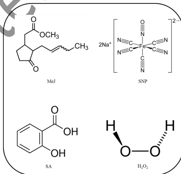
Fig. 2: Elicitor chemical structures, MeJ: methyl jasmonate; SNP: sodium nitroprusside, a donor of nitric oxide; SA: salicylic acid and H 2 O 2 : hydrogen peroxide
