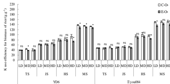
Fig. 2: Effects of surface ozone concentration and plant density on K use efficiency for biomass of rice under FACE condition
