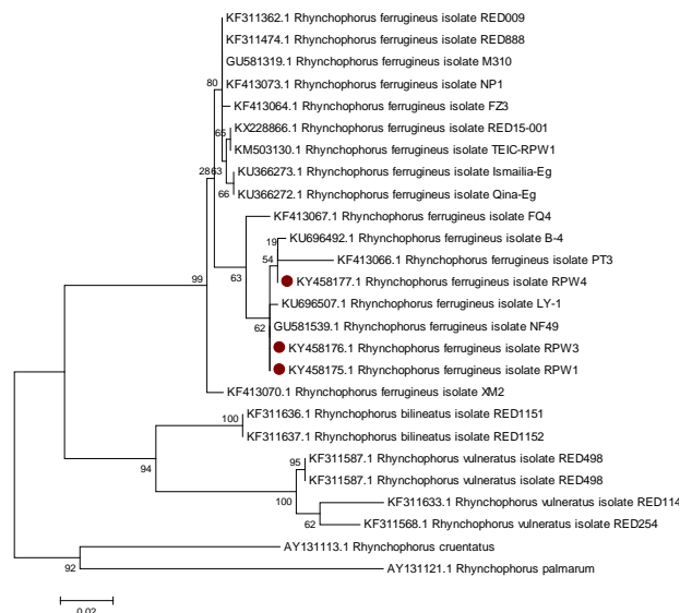
Fig. 3: Phylogeny tree based on COI produced by Maximum Likelihood Method using MEGA6 according to according to Tamura et al. , (2013)
