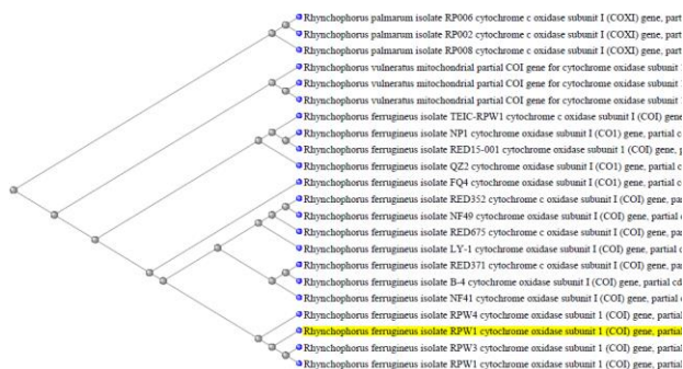
Fig. 4: Maximum parsimony tree constructed through BLAST pair base alignment
