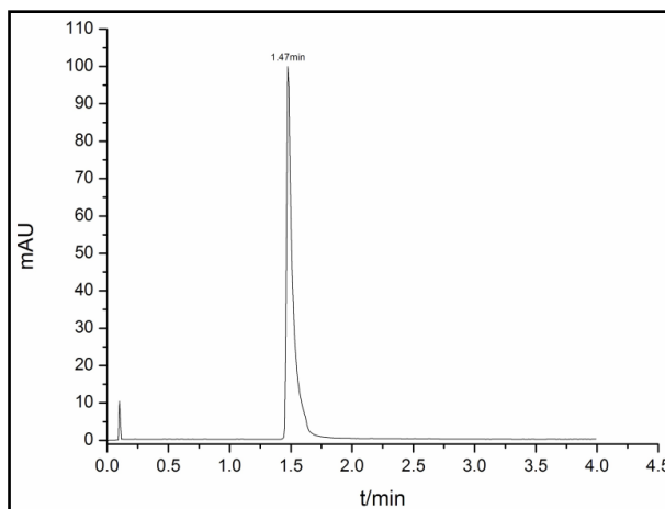
Fig. 6: Chromatogram of difenoconazole standard solution
