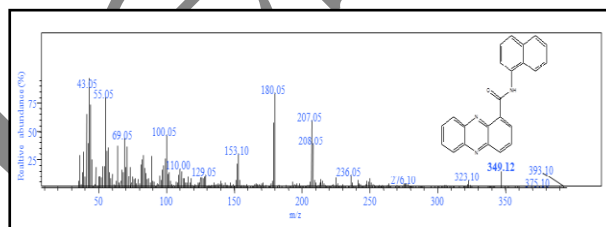
Fig. 5: Mass spectrum of PCND 18-1
