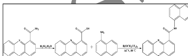
Fig. 2: Synthesis of PCND 18-1
