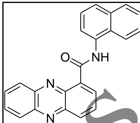
Fig. 1: Structural formula of PCND 18-1
