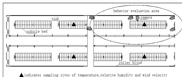
Fig. 1: The sampling sites of ambient temperature, relative humidity and wind velocity in the cowshed
