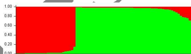
Fig. 6: Population structure analysis of wild rhubarb genotypes and R. rhubarbarum cultivar using SSR markers
