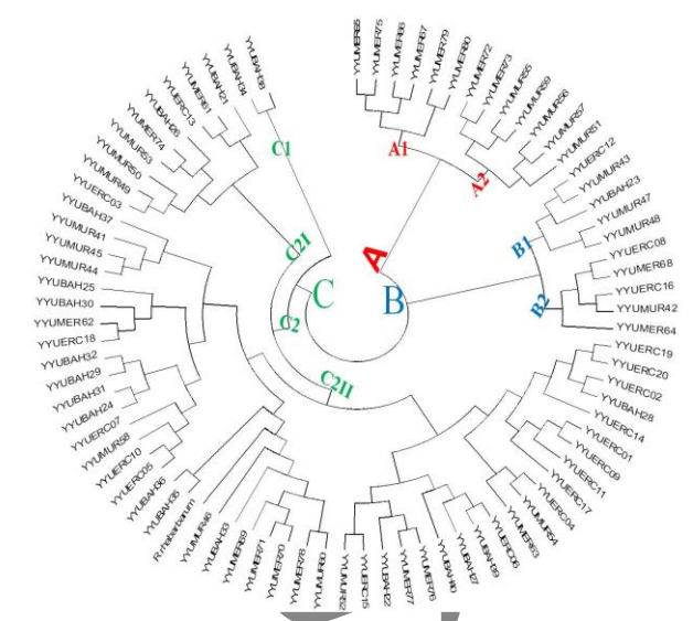
Fig. 1: Neighbor joining clustering of 80 wild rhubarb genotypes and R. rhabarbarum cultivar using ISSR markers
