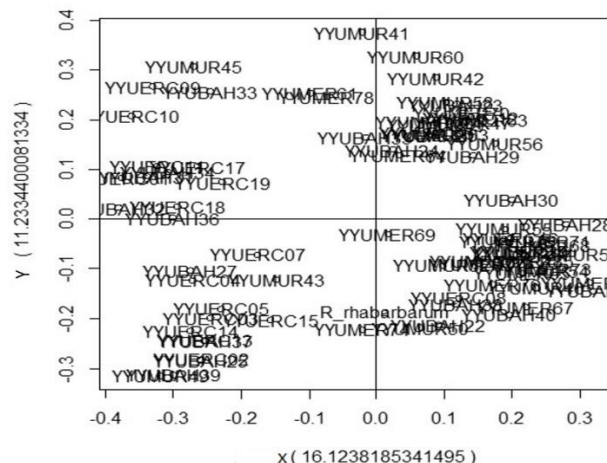
Fig. 5: Jaccard similarity analysis of 80 wild rhubarb genotypes and R. rhubarbarum cultivar using SSR markers
