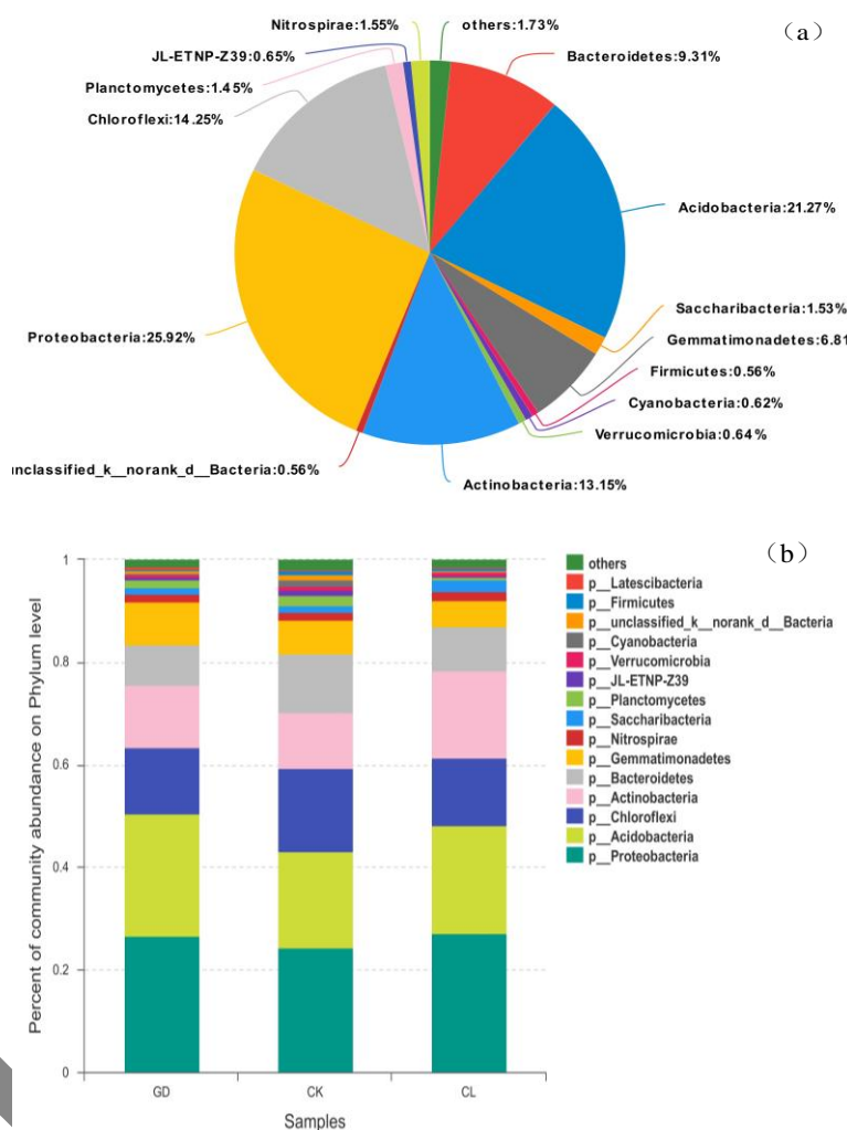
Fig. 1: (a). Relative abundances of soil bacterial phyla from the total soil samples; and (b). Different soil samples (CK: saline soil; GD: farmland soil; and CL: improved saline soil)
