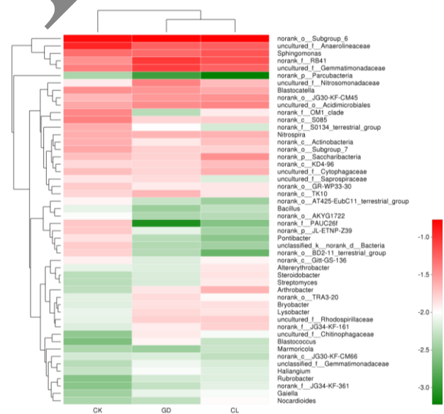
Fig. 3: The results of the clustering analysis as a heatmap of the three soil types
